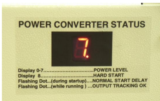
A converter under heavy load
